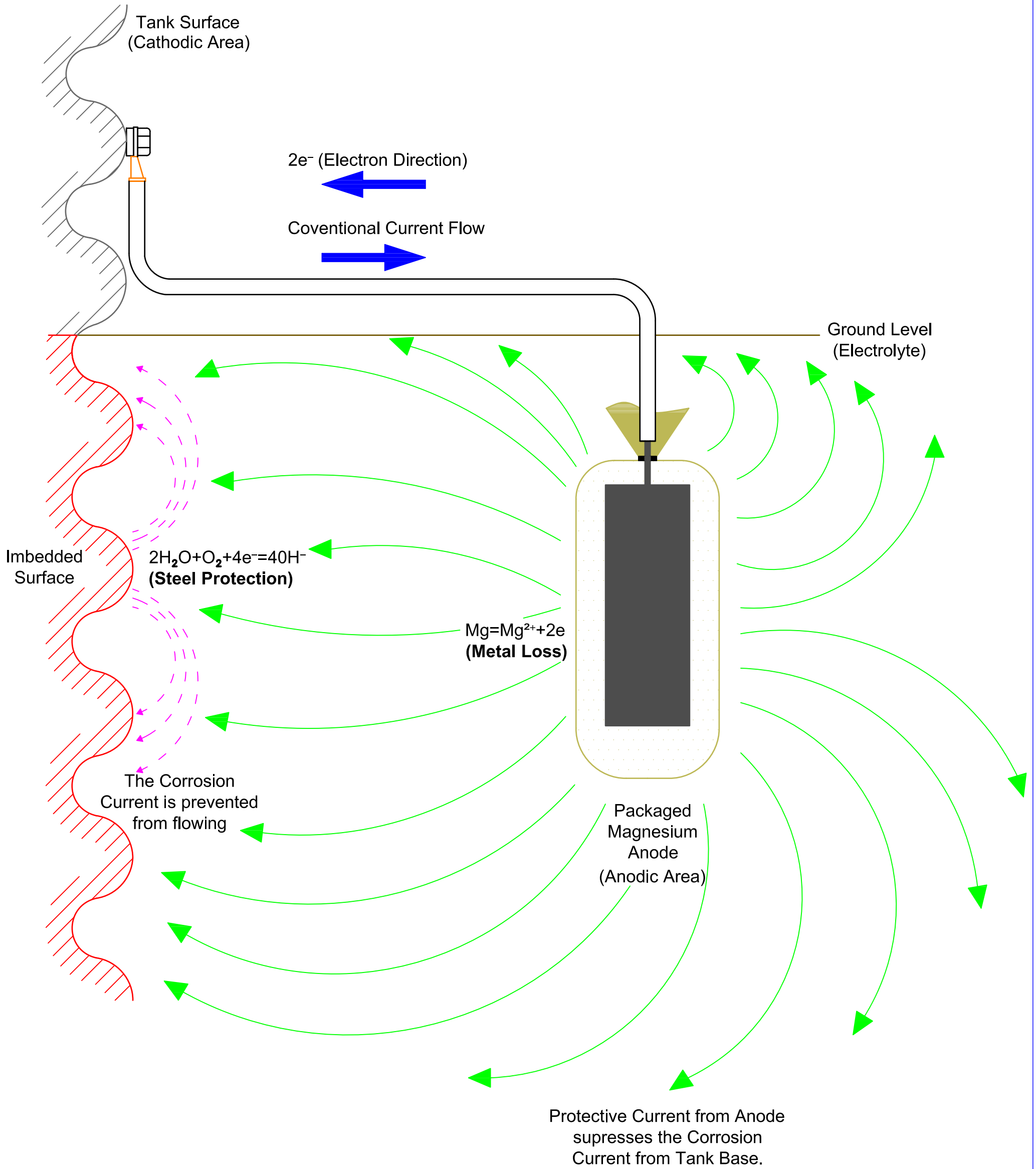
Figure 1.4 Close-up view of the Tanks base with Cathodic Protection.
