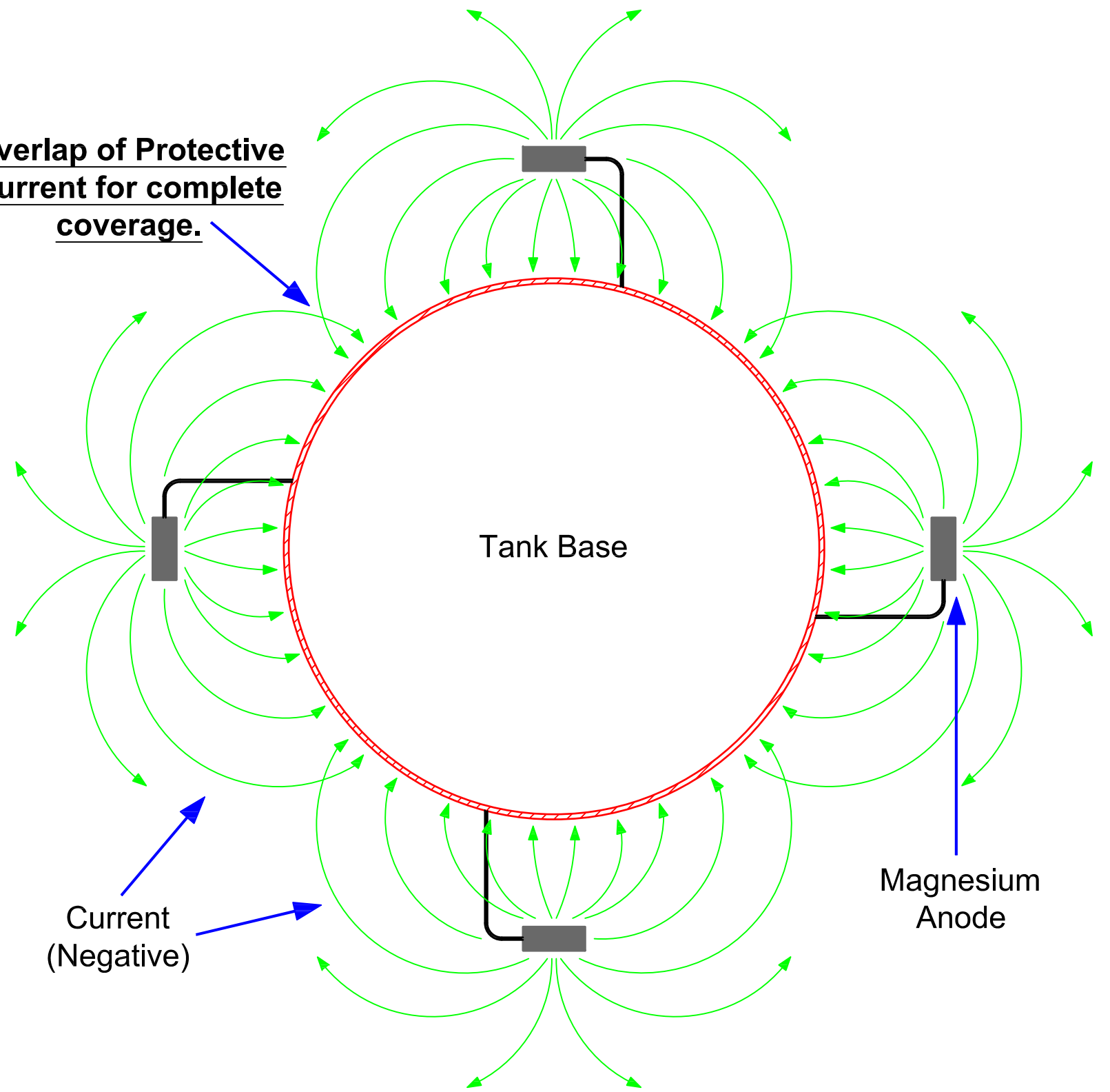
Figure 1.3 Top View - Base of Tank with Cathodic Protection
