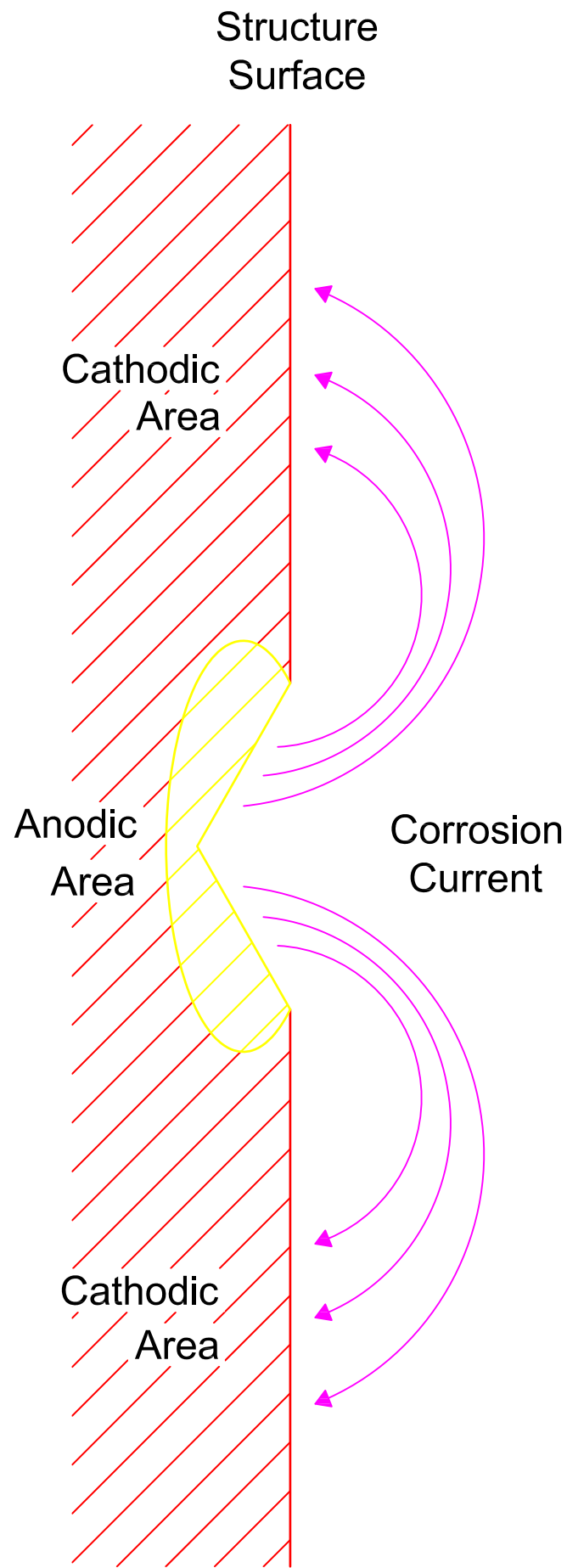
Figure 1.2 Close-up view of the Corrosion Process.
